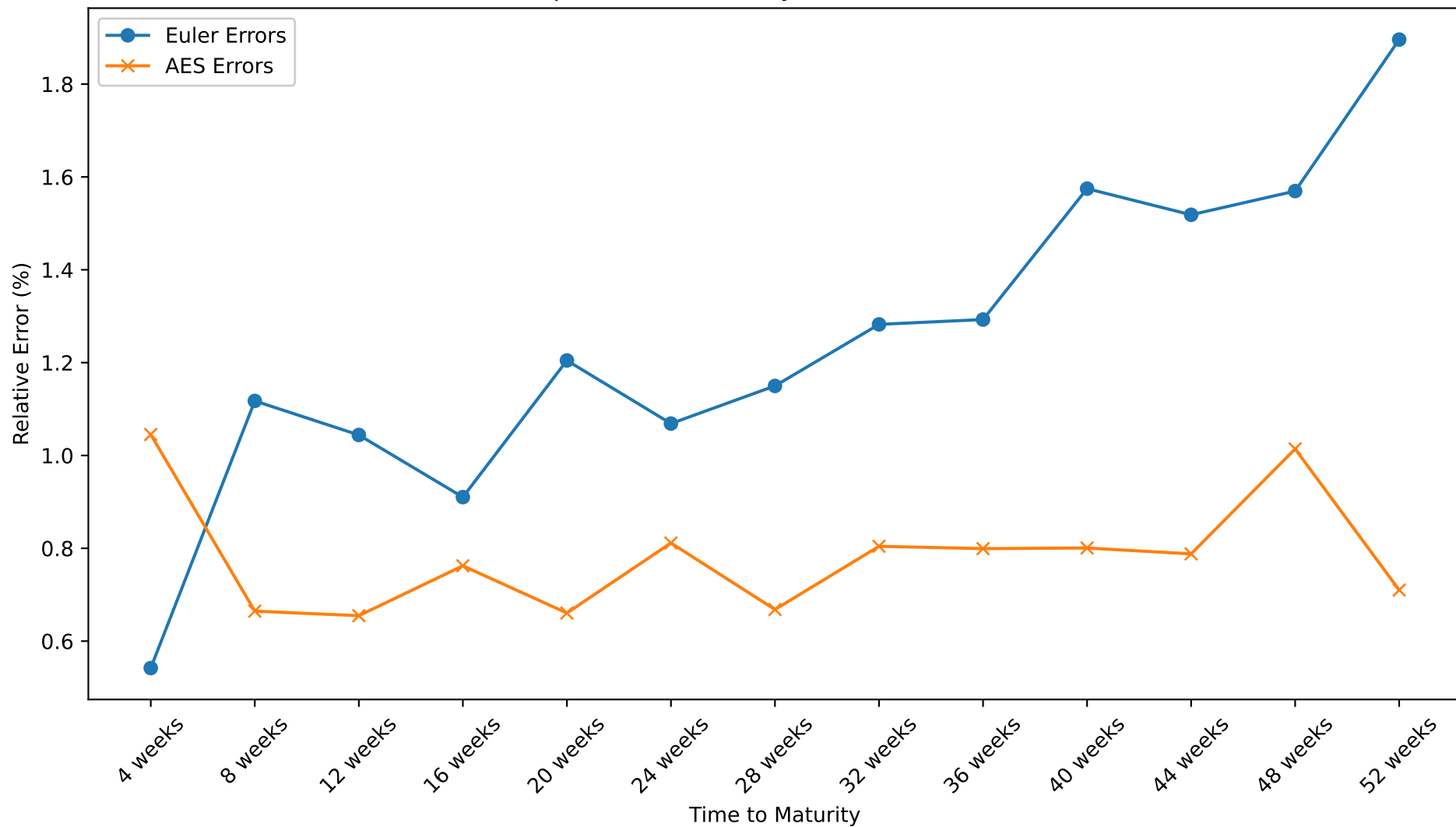
Bermuda Option with biweekly Exercise Dates for S_0=100
